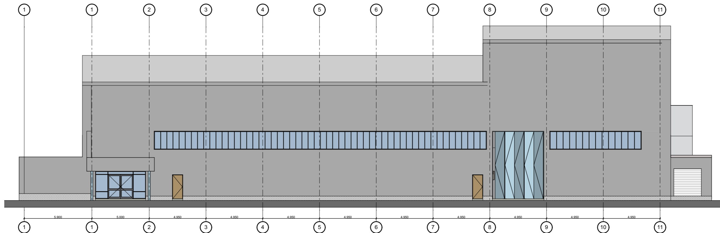
West Elevation
