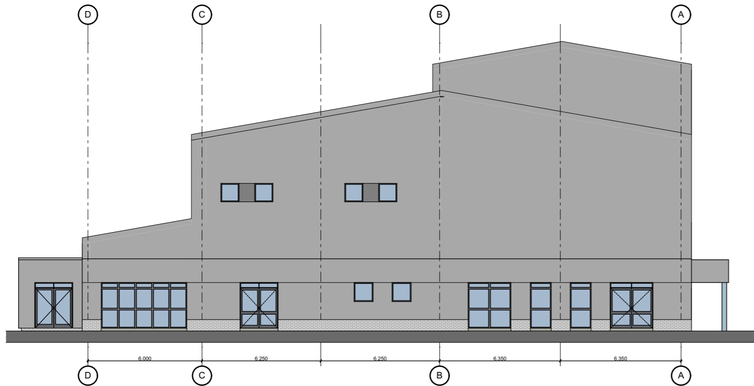
North Elevation
