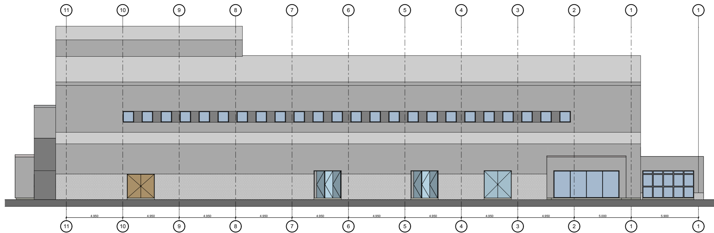
East Elevation
